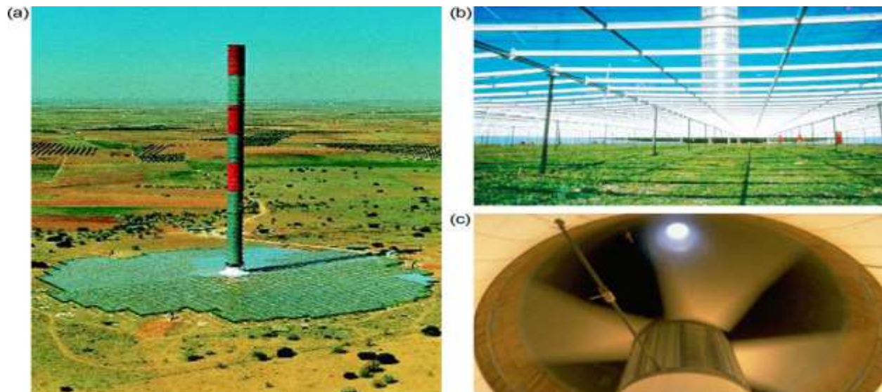
Figure 1. Pictures of Manzanares plant prototype: (a) whole plant; (b) collector; (c) turbine (Schlaich et al. , 2005).
