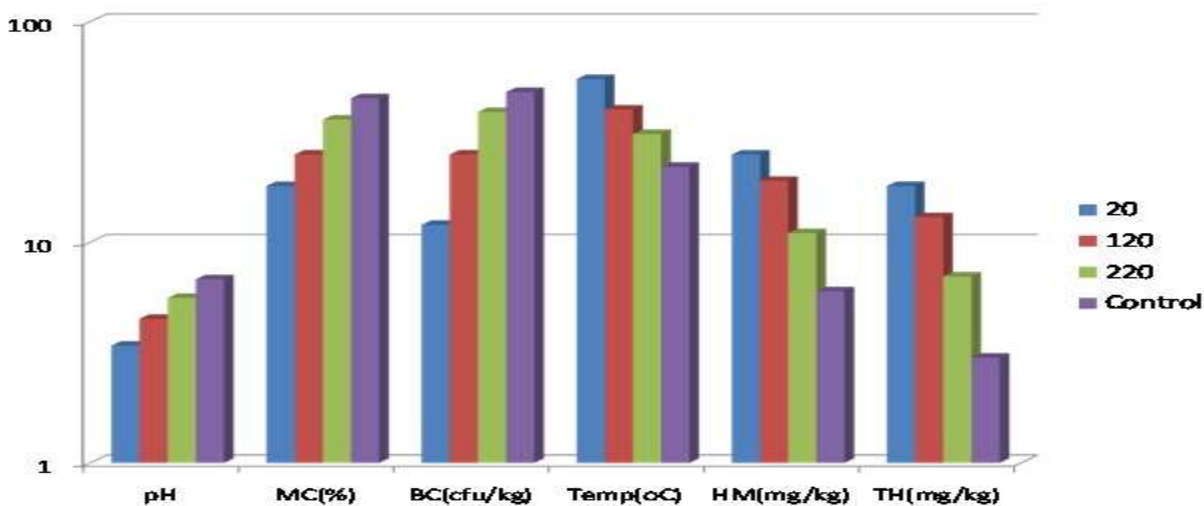
Figure 5: Multiple Bar Chart Showing the Relationship between Concentration of pH, Moisture Content (MC), Bacteria Count (BC), Temperature, Heavy Metals (HM) and Total Hydrocarbon (TH) in Soil and Distance from a Gas Flaring Station.
