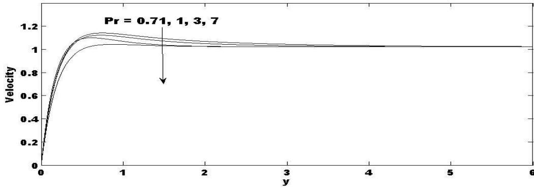
Figure 8. Velocity profiles for different values of Pr.
