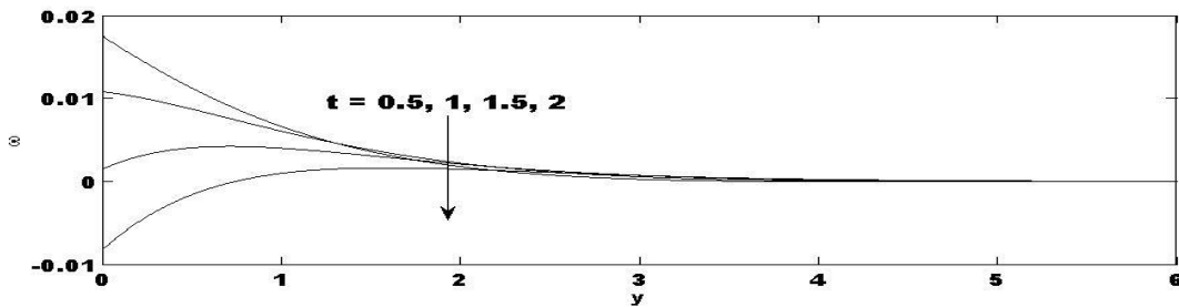
Figure 6. Angular velocity profiles for different values of t .
