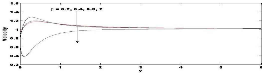
Figure 13. Velocity profiles for different values of \beta .
