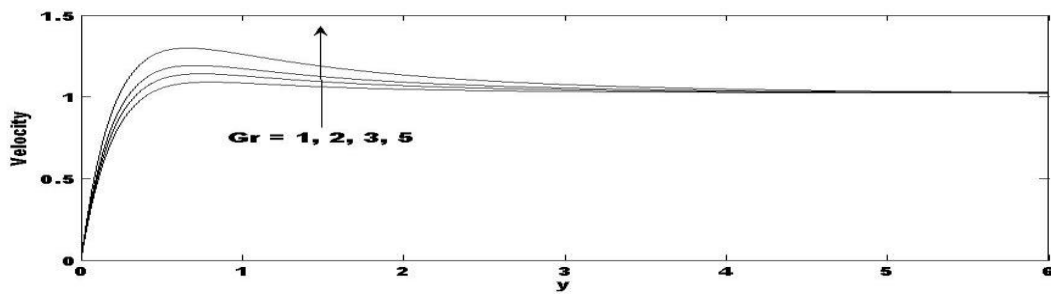
Figure 9. Velocity profiles for different values of Gr.
