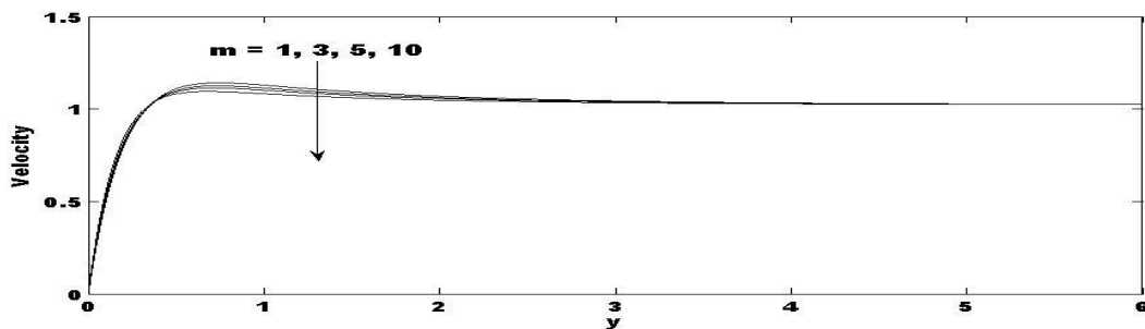
Figure 14. Velocity profiles for different values of m .
