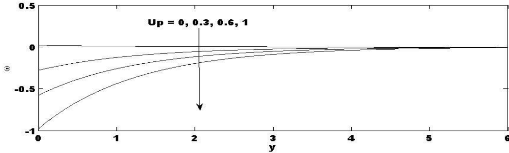
Figure 4. Angular velocity profiles for different values of U_p .
