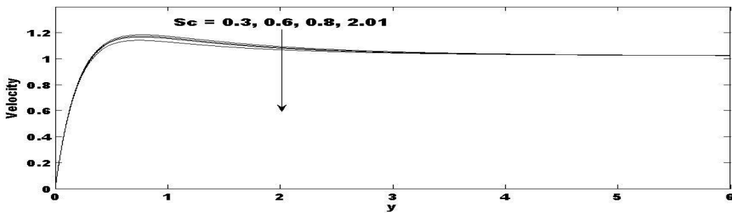
Figure 7. Velocity profiles for different values of Sc .
