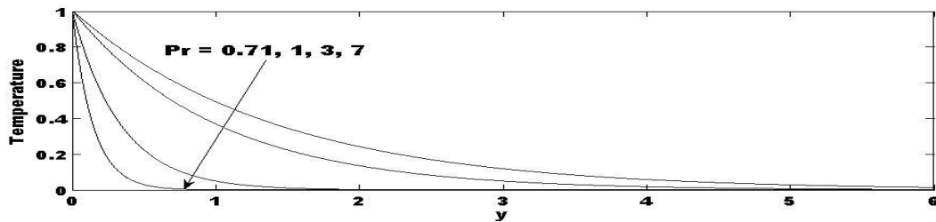
Figure 1. Temperature profiles for different values of Pr .
