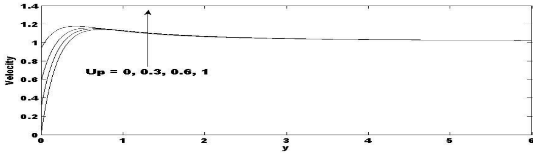
Figure 12. Velocity profiles for different values of U_p .
