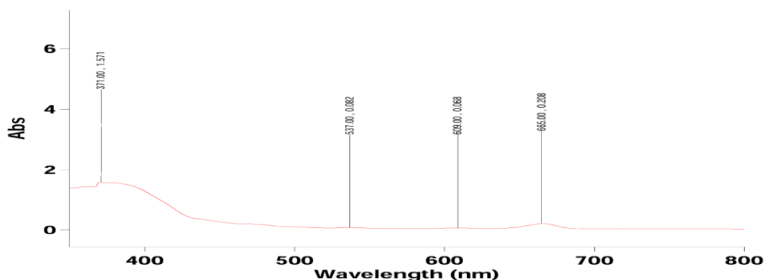
Figure 1: FTIR of crude methanol extract
